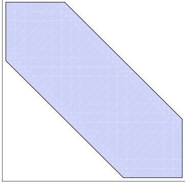
Figure 1: Sumfree region for k = 2
