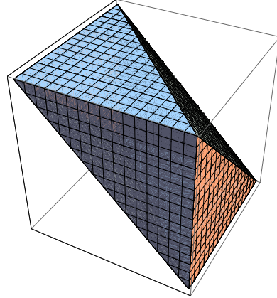
Figure 2: Sumfree region for k = 3
