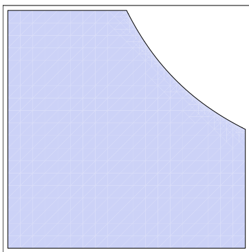
Figure 3: Method of Theorem 5.3
