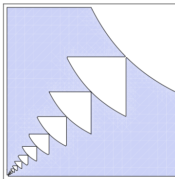
Figure 4: Method of Theorem 6.1
